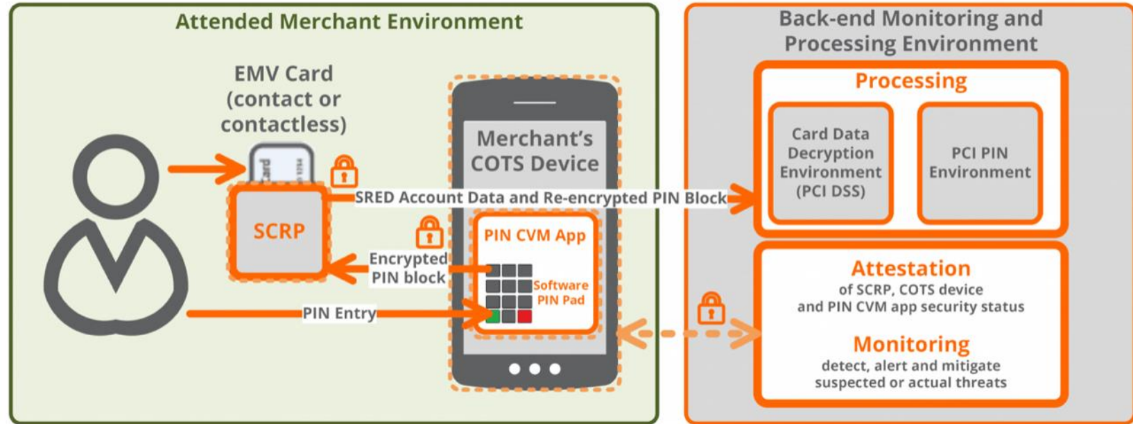
Figure 1: High-level view of a SPoC Solution
