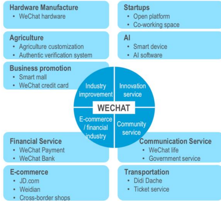
Figure 34. Tencent Ecosystem
